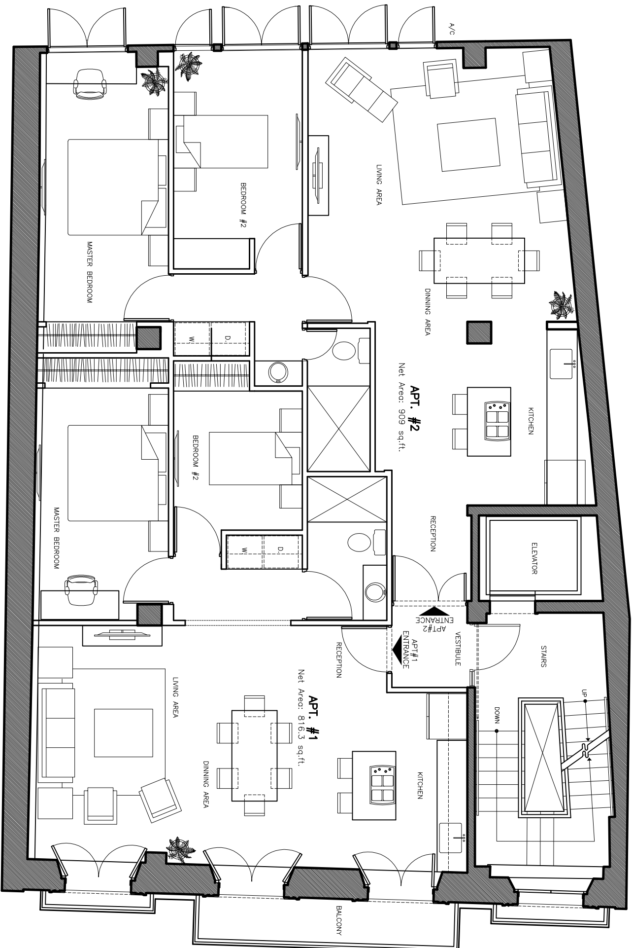
Proposed Second Floor Plan (Rev. 1) Scale: 3/16"=1'-0"
